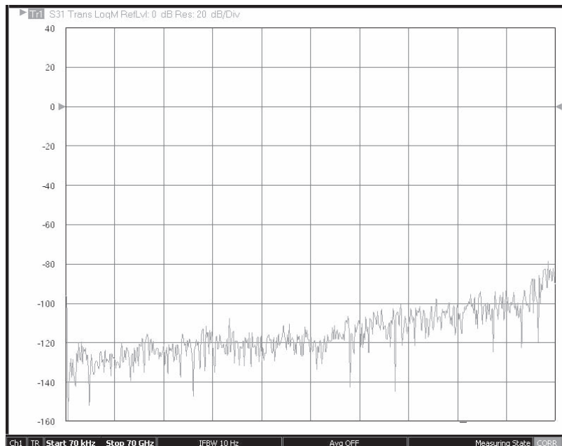
System Dynamic Range (As Measured, not RMS). 10 Hz IF BW, No averaging, at max power. Ports terminated after Transmission Cal.
