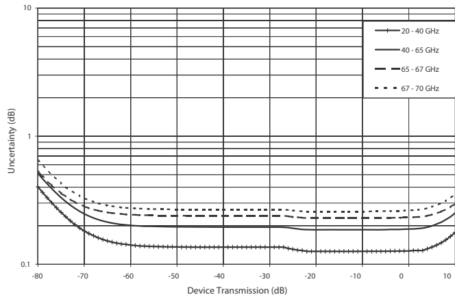
Transmission Magnitude Uncertainty (2 of 2) MS4647A with SOLT Calibration using 3654D Cal Kit
